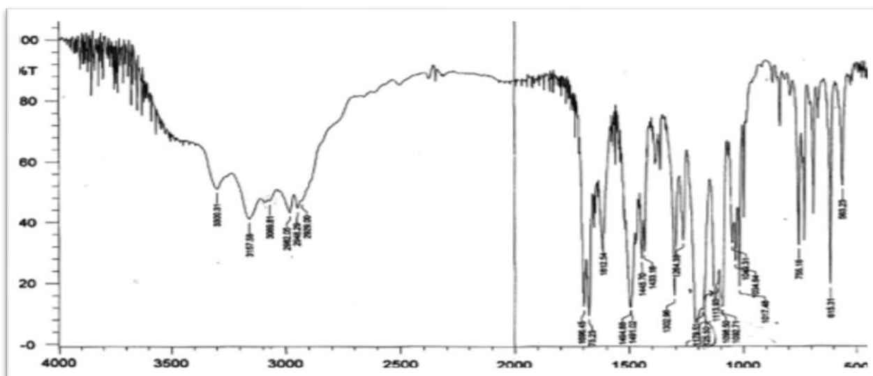
Figure 5. FT-IR of Amlodipine Besylate
