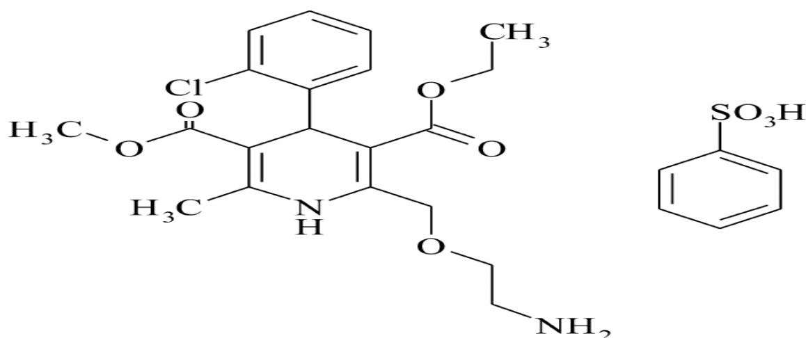
Figure1. Structure of Amlodipine besylate
